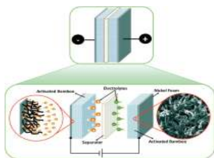
Fig. Schematic diagram of supercapacitor device and its individual components
