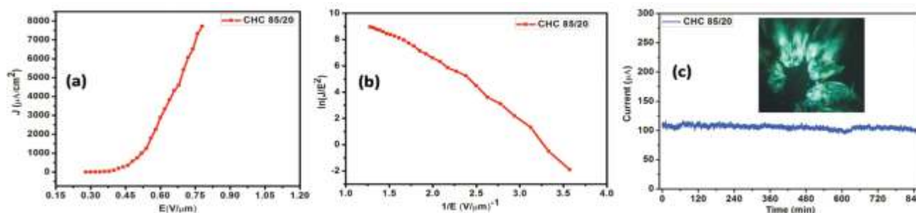
Fig. 3 Field emission characteristics, (a) current density (J) as a function of applied electric field (E), (b) F-N plot \{\ln(J/E^2)\} versus 1/E , (c) field emission current stability (i-t) plot and the corresponding field emission image (inset).
