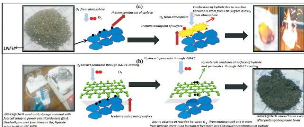
Fig. Schematic representation of (a) burning of LNFH without rGO-EC encapsulation (b) selective permeability of rGO-EC in rGO-EC@LNF.
